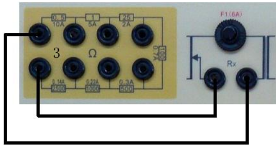
Figure 5-2 String into seven 50W resistors
