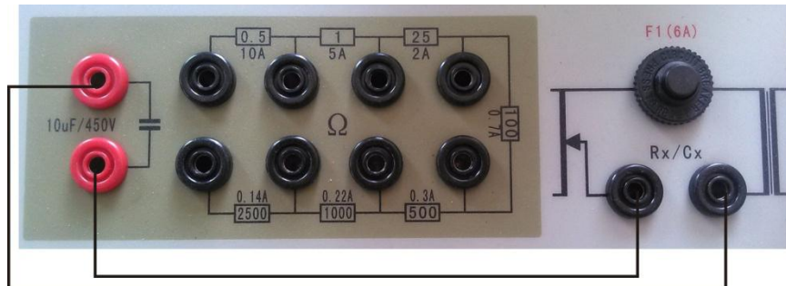
Figure 5-3 String into capacitors
