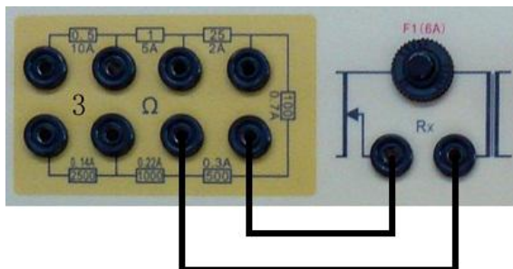
Figure 5-1 String into a resistor 500 ohm/50W
